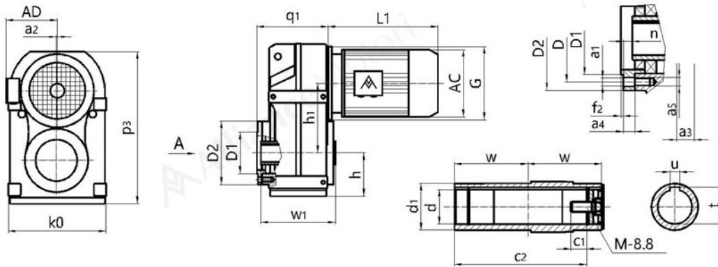
(Fig.A Mounting Dimension)
