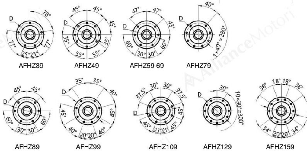
(Fig.A Mounting Dimension)
